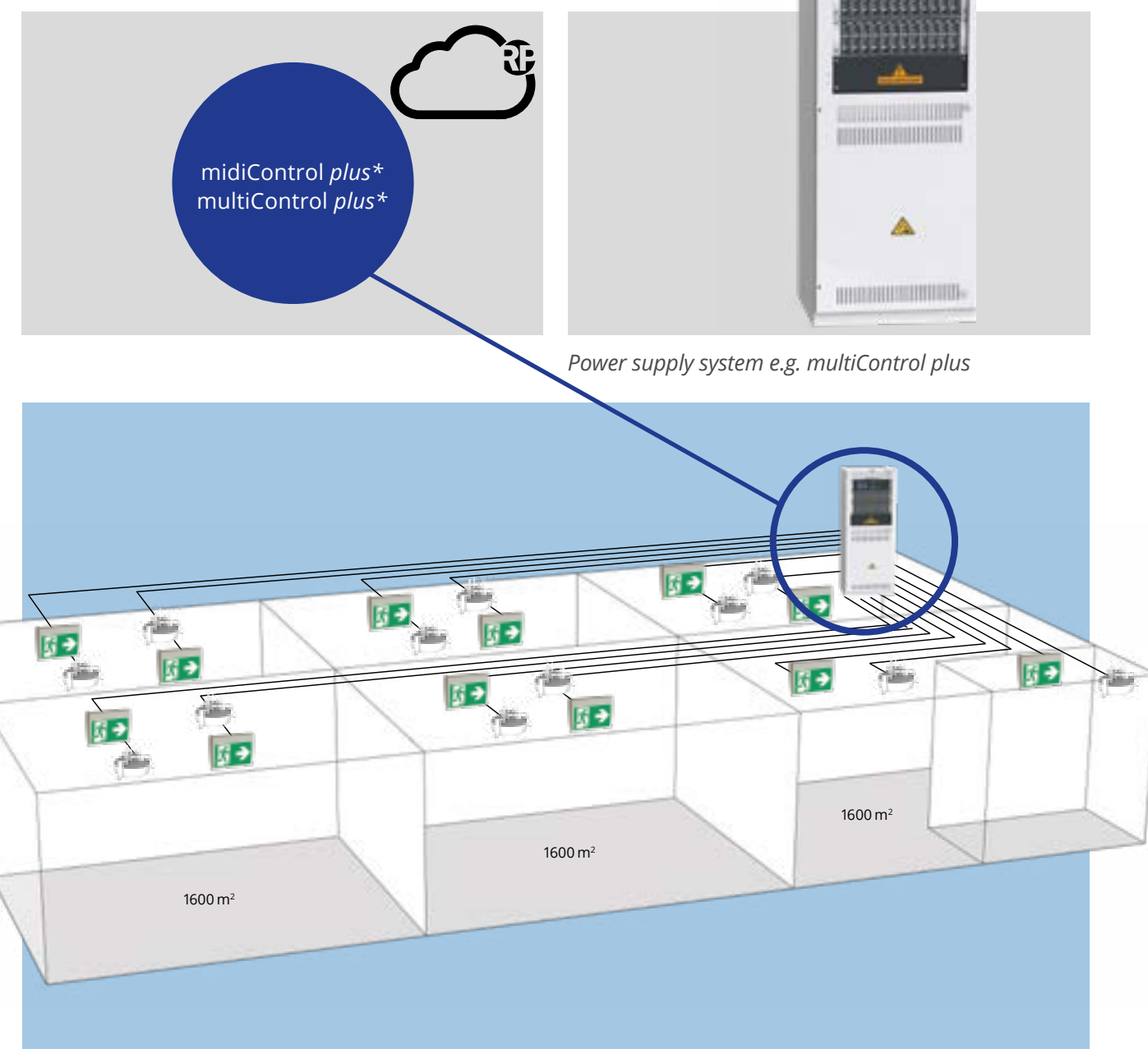
Example of an industrial building with virtual fire compartments
