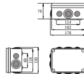
IP 54
